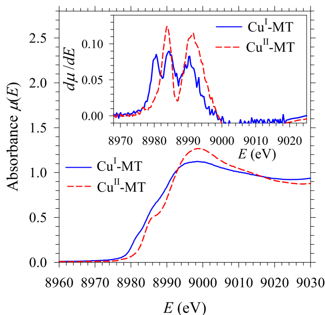
FIGURE 5 XANES data of Cu I -MT and Cu II -MT. ( Inset ) The corresponding d\mu/dE profiles.
