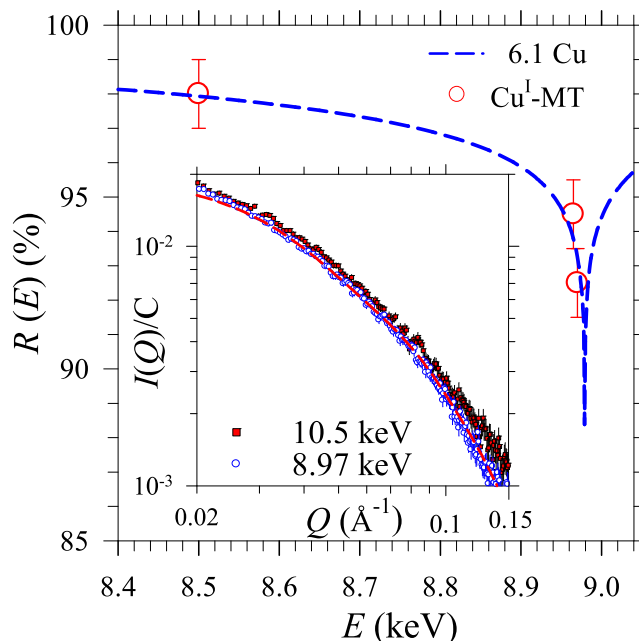
FIGURE 4 The R(E) values of Cu I -MT measured at 8.5, 8.965, and 8.970 keV, with E_{\text{ref}} = 10.5 keV, are fitted with 6.1 Cu ( dashed curve ) using Eq. 2. ( Inset ) ASAXS data measured at 10.5 and 8.970 keV. The 8.970 keV data are fitted with a rodlike model ( dashed curve ). For clarity, ASAXS data measured with 8.5- and 8.965-keV x-rays are not shown.
