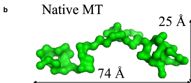
FIGURE 1 (a) SAXS data of the native MT (10 mg/ml) and unfolded apo-MT (2.5 mg/ml) are fitted with a rodlike shape (upper dashed curve) and power-law scattering I(Q) \propto Q^{-1} (lower dashed line), respectively. Also shown are the SAXS data of the refolded apo-MT (10 mg/ml). All data were collected with 10.5-keV x-rays. (Inset) Guinier approximations (dashed lines) for the SAXS data of the native MT and refolded apo-MT (solid and long-dashed lines indicate the higher- and lower-bound R_g values). (b) Protein envelope of the native MT obtained from the dummy-residue simulation with the SAXS data.
